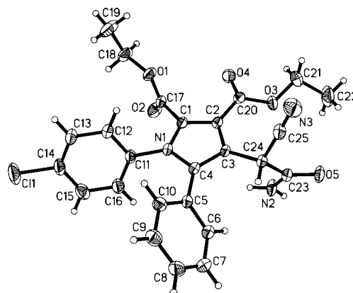
Figure 1. X-ray structure of compound 5ar .
